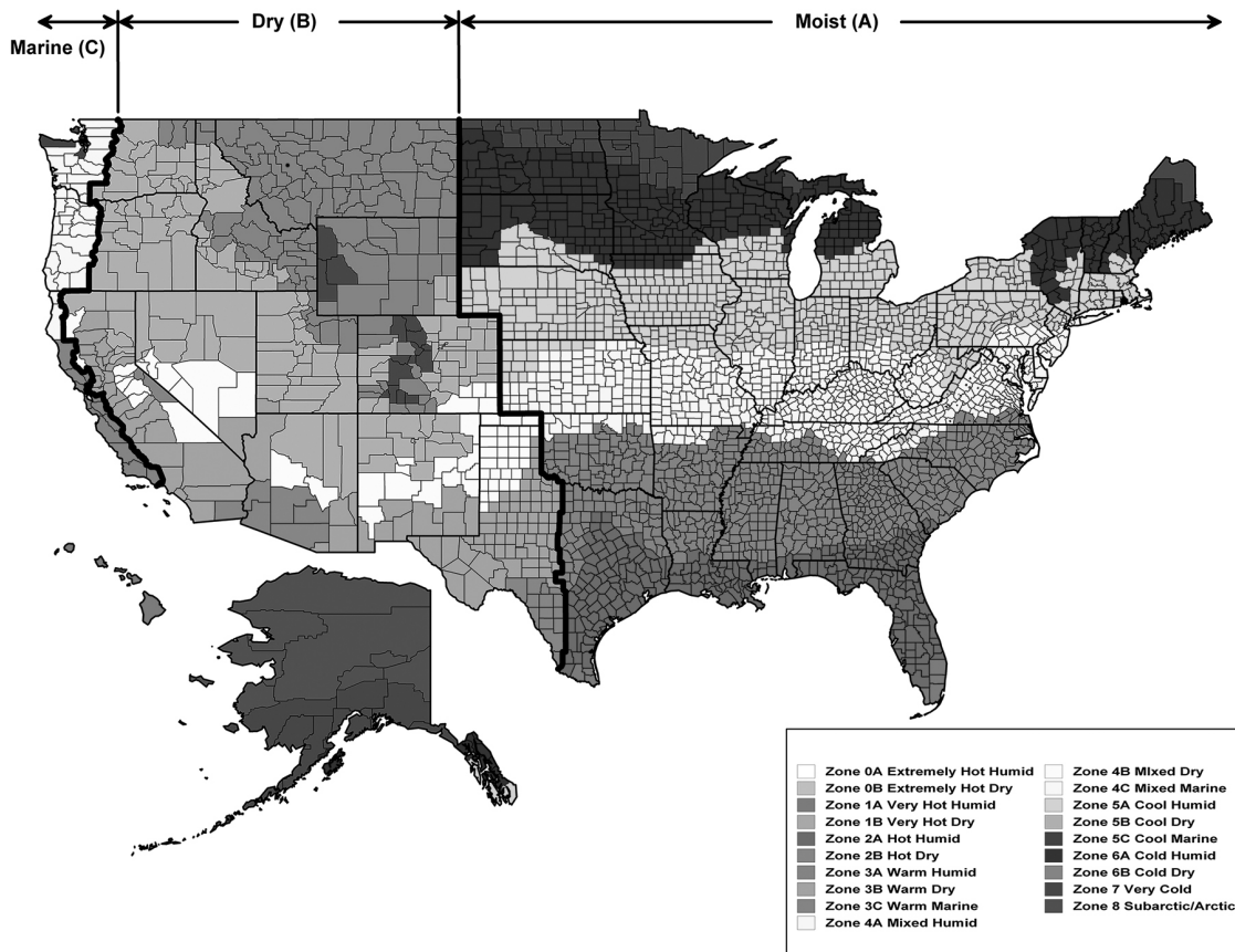
FIGURE 302.2.2.2.1 CLIMATE ZONE MAP
