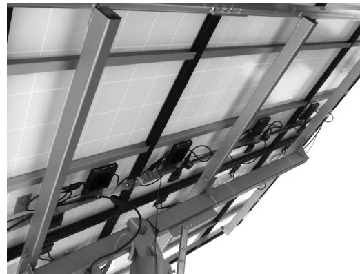
Figure 5: Example Microinverter
